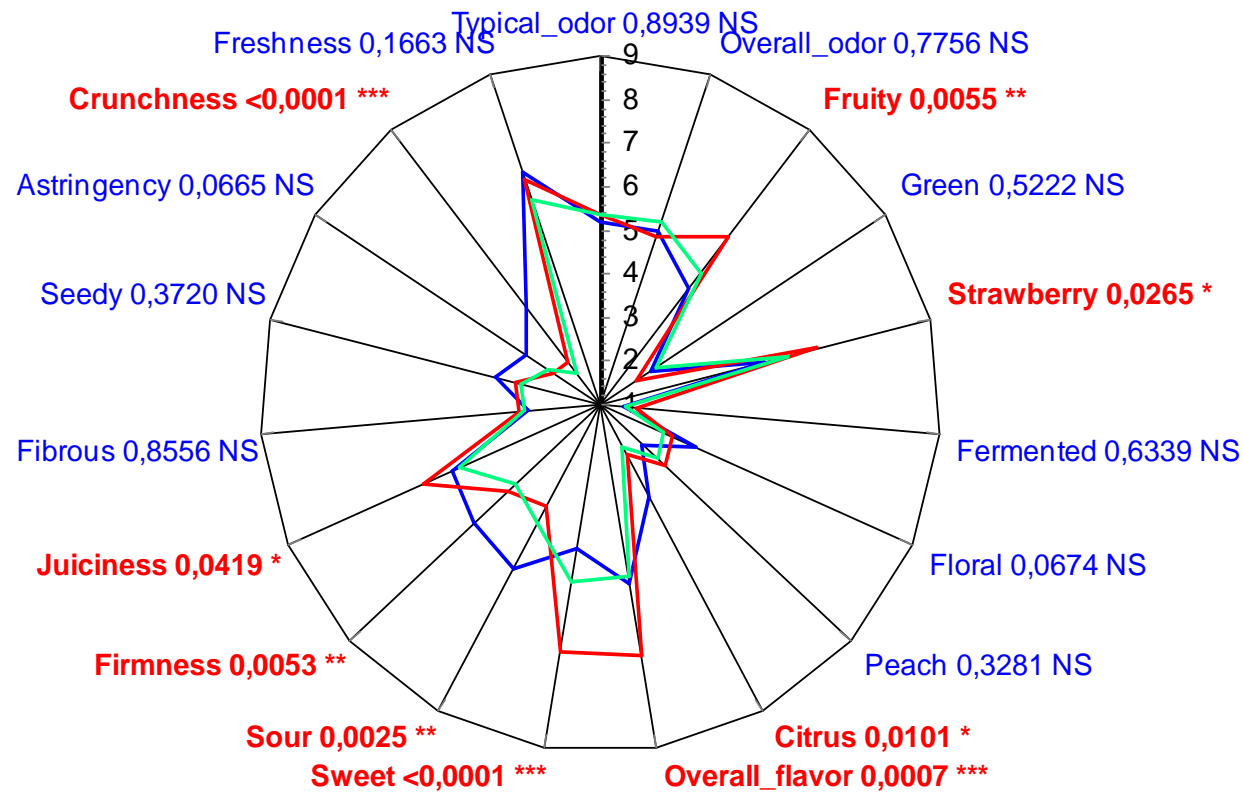
Profile Strawberry profile File: descriptive_analysis.frs Statistics computation: global Plot of: Mean Analysis of variance
